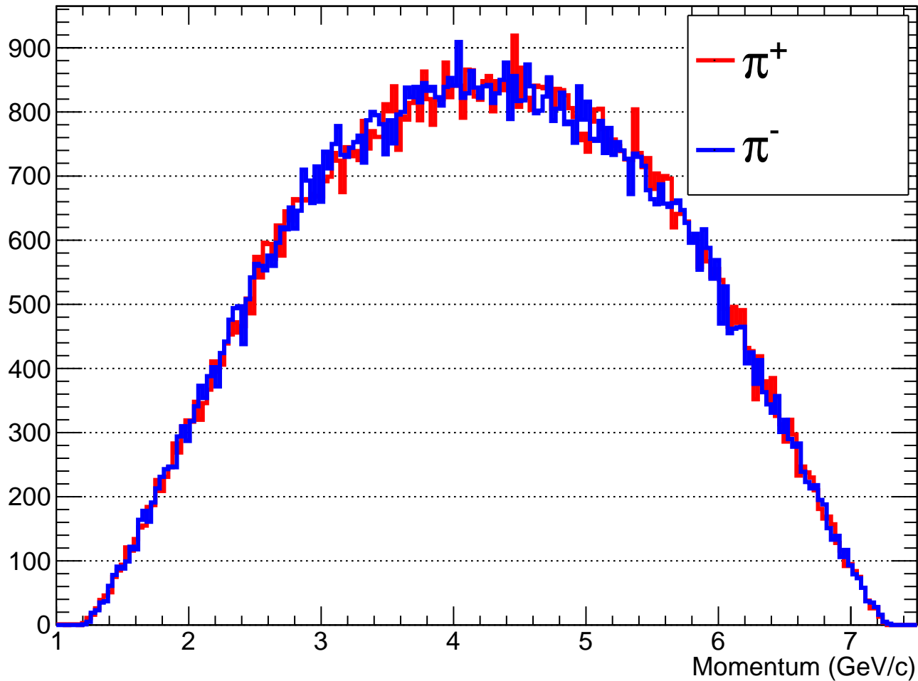
\pi^\pm momentum distribution in lab frame
