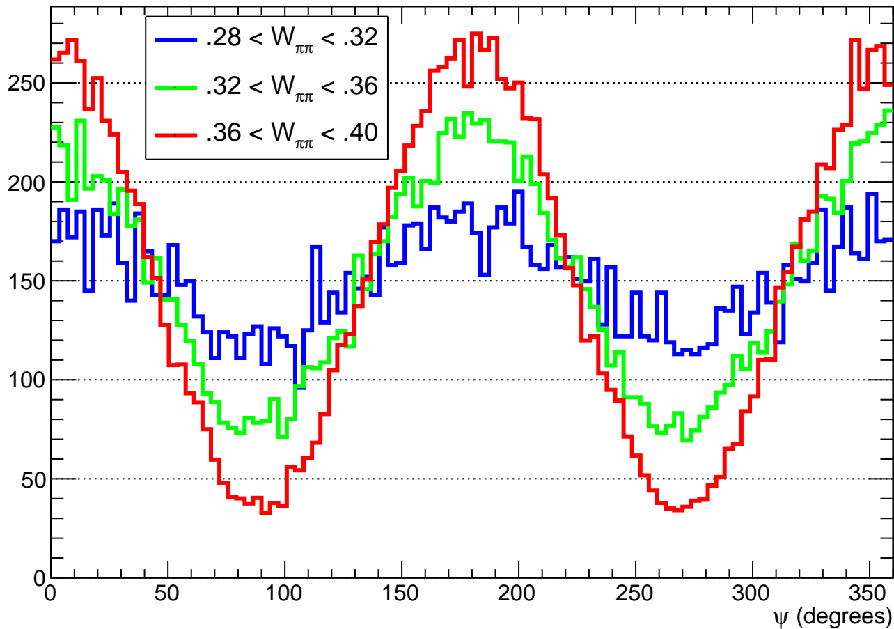
\pi\pi scattering plane angle wrt proton scattering plane in \pi\pi CM frame
