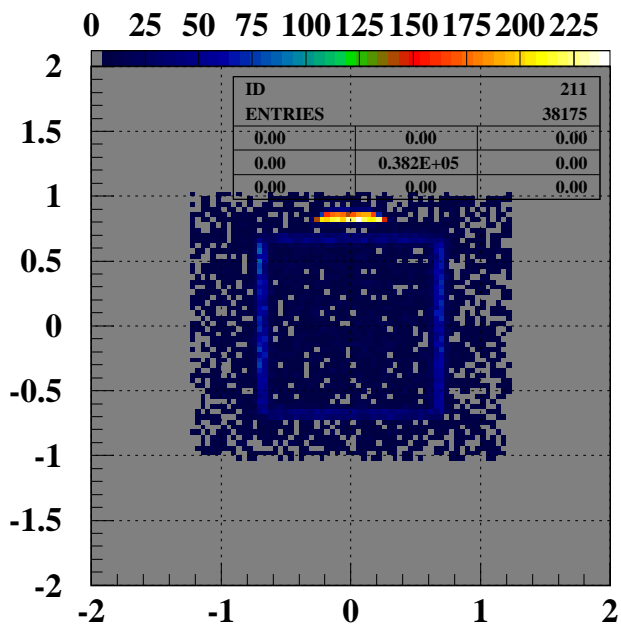
Exit y vs x (failure)
