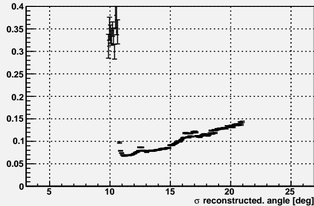
BCAL \sigma Reconstructed angle vs. generated angle
