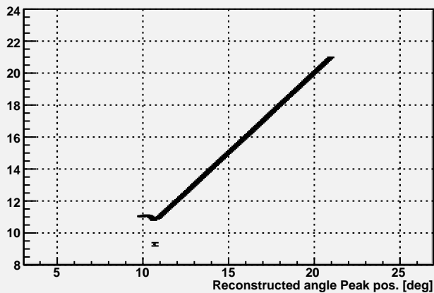
BCAL Reconstructed angle vs. generated angle
