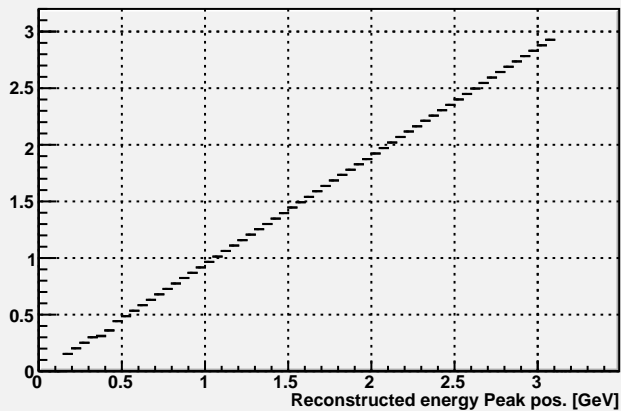
BCAL Reconstructed energy vs. generated energy [GeV]
