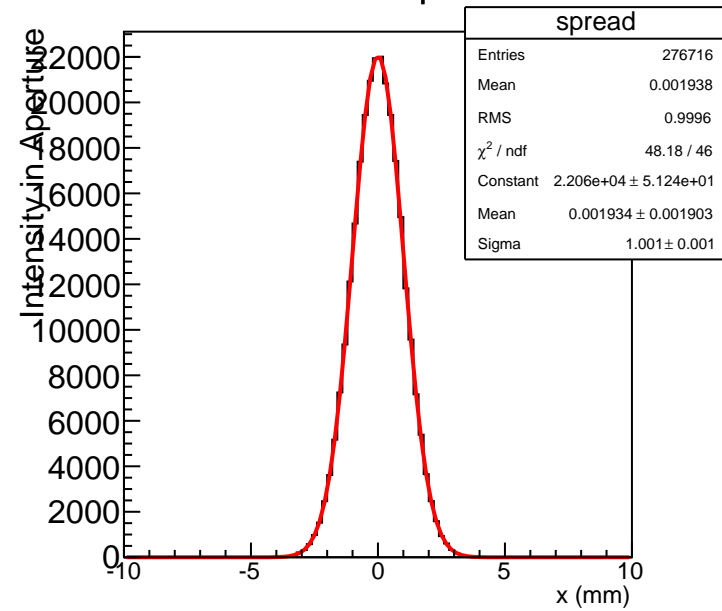
Gaussian spread
