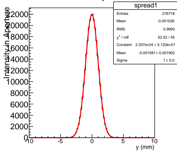
Gaussian spread
