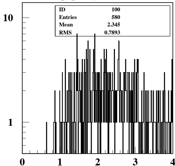
fcal only photons
