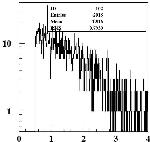
fcal and bcal photons
