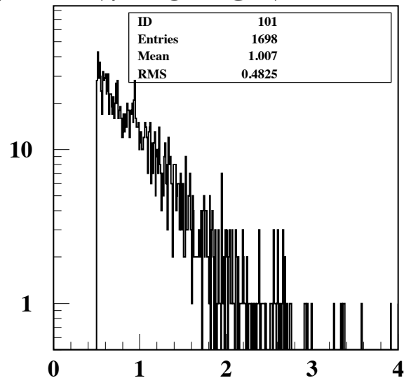
bcal only photons
