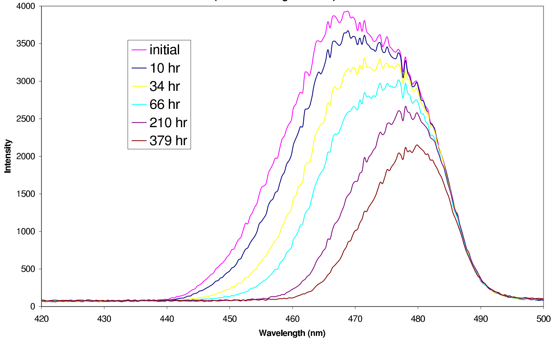
Intensity Degradation of a PoliHiTech Scintillating Fiber as a Result of UV Light Exposure (470 nm LED light source)
