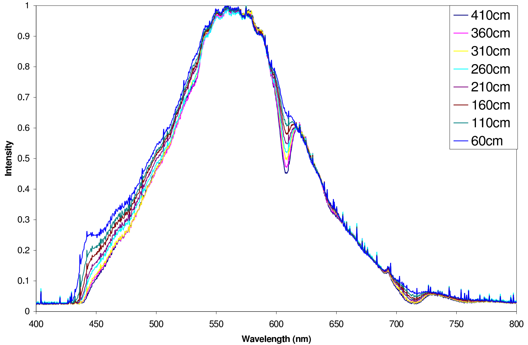
Normalized (Average) Signal Intensity as a Function of Scintillating Fiber (Pol.Hi.Tech) Length
