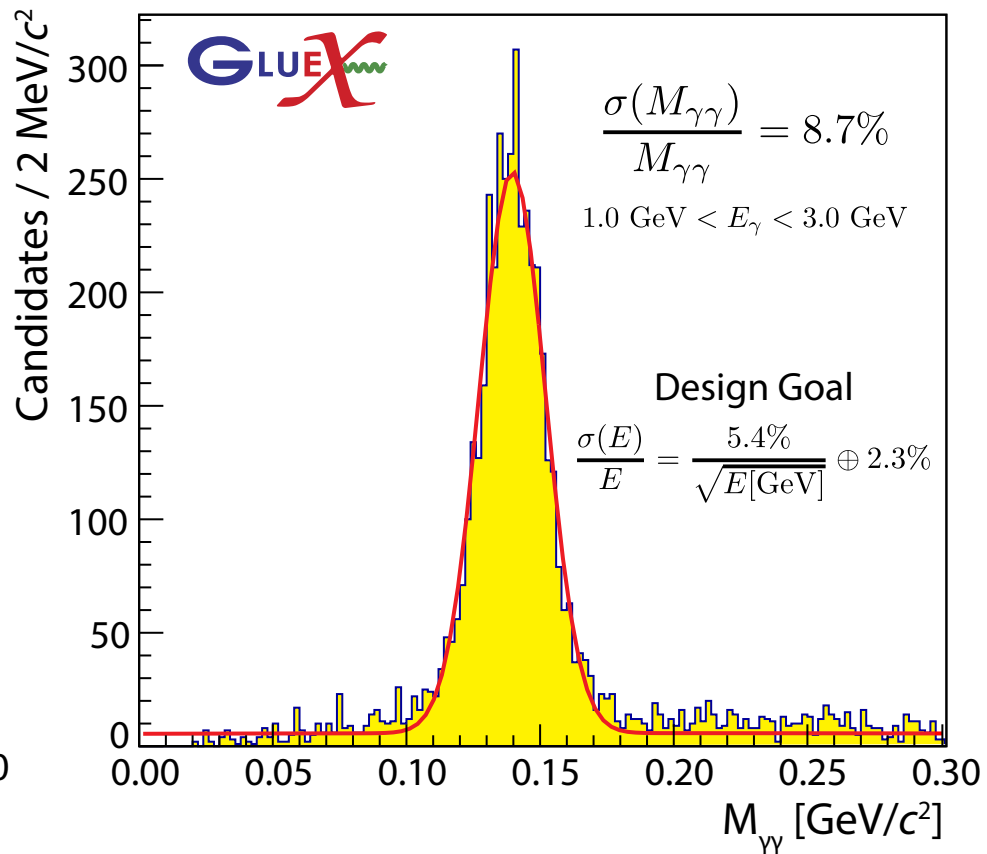
Barrel Lead-Scintillating Fiber Calorimeter
