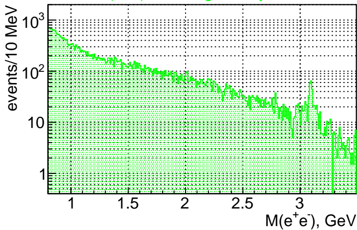
M(e^+e^-) from angles only
