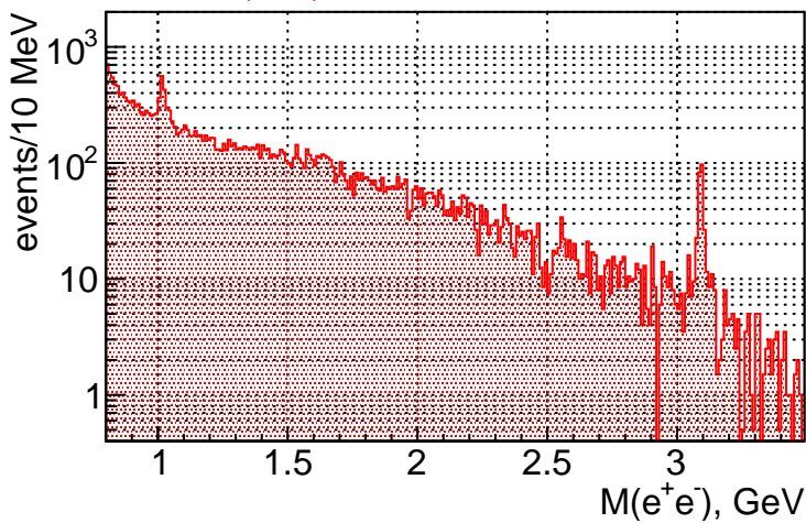
M(e^+e^-) from kinematic fit
