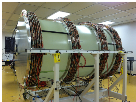
Figure 6. The GlueX Forward Drift Chamber (FDC) assembled and ready for final testing. The FDC consists of four separate packages, each with six chambers. Each chamber provides signals both from the wires and the cathode strips. Both the upstream and downstream cathode planes are instrumented for readout. This provides information on the position along the hit wire improving the pattern recognition.
