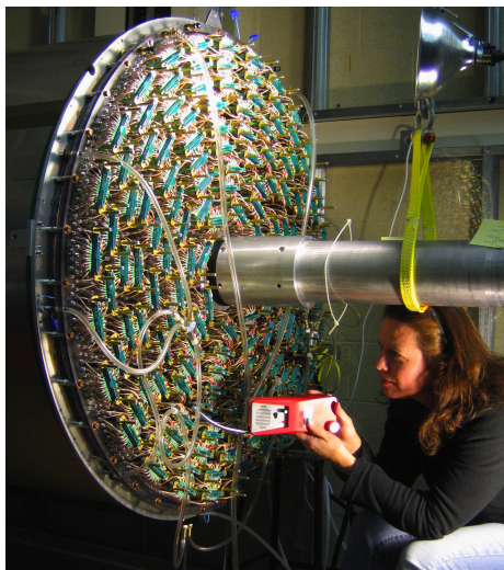
Figure 5. Central Drift Chamber (CDC) being tested for gas leaks. The CDC is a straw tube drift chamber with approximately 3500 straw tubes. It is made from alternating sections of axial (parallel to the beam direction) and stereo ( 6^\circ angle with respect to the beam direction). This allows the track's polar angle ( \theta ) to be determined when multiple layers are considered. The end plate shown is populated with the amplifier electronics which instrument the wires to the left.
