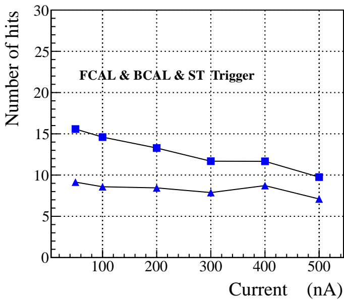
Multiplicity (BG subtracted)
