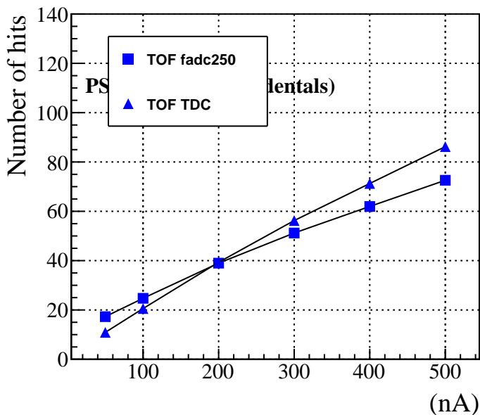
Multiplicity (BG subtracted)
