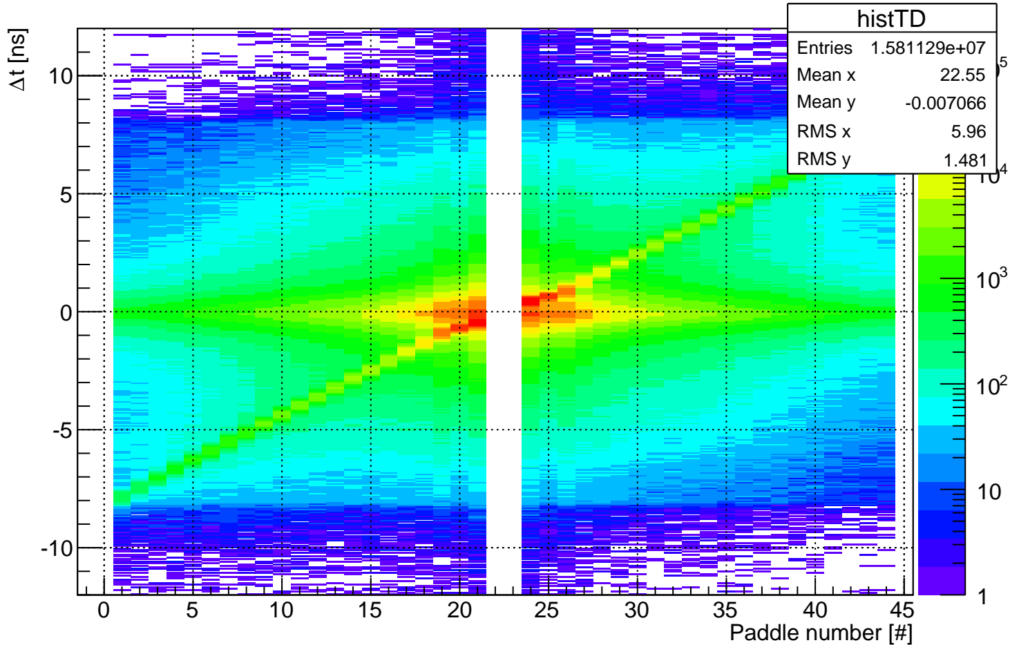
Paddle number other plane vs. \Delta t Paddle REFPAD21
